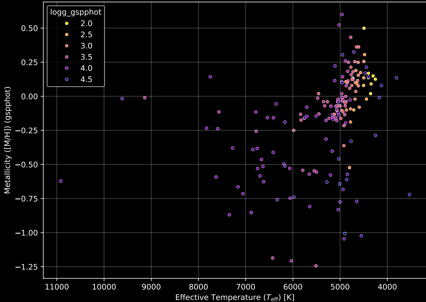
APOGEE DR17 Field: [LMC12] Stellar Population Parameters (n= 175)
