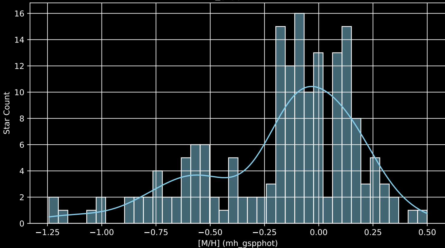
APOGEE DR17 Field: [LMC12 [M/H] (mh_gspphot) (n= 173)
