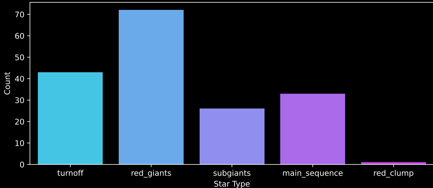
APOGEE DR17 Field: [LMC12] Count plot of Star Type
