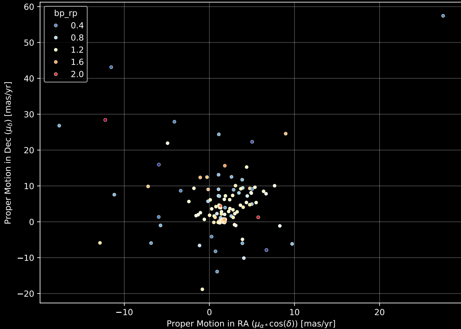
APOGEE DR17 Field: [LMC12] Proper Motion Diagram (n= 175)
