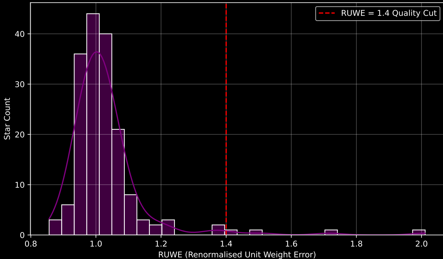
GAPOGEE DR17 Field [LMC12] RUWE Distribution (n= 172)
