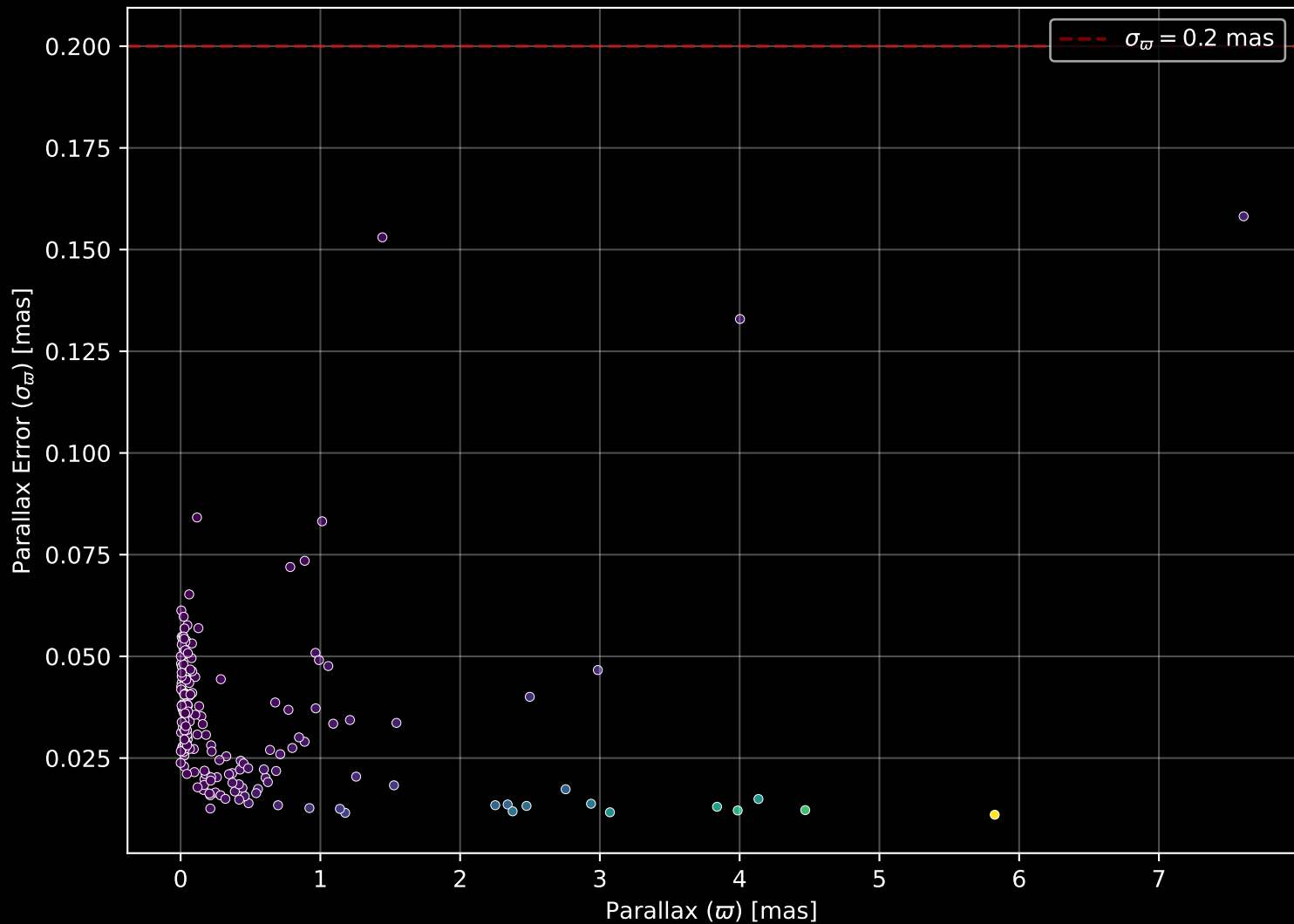
APOGEE DR17 Field: [LMC12] Parallax Quality (n= 175)
